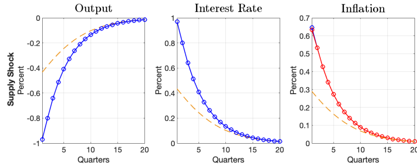
Figure 4: Impulse Responses of Inflation and Household Inflation Expectation
